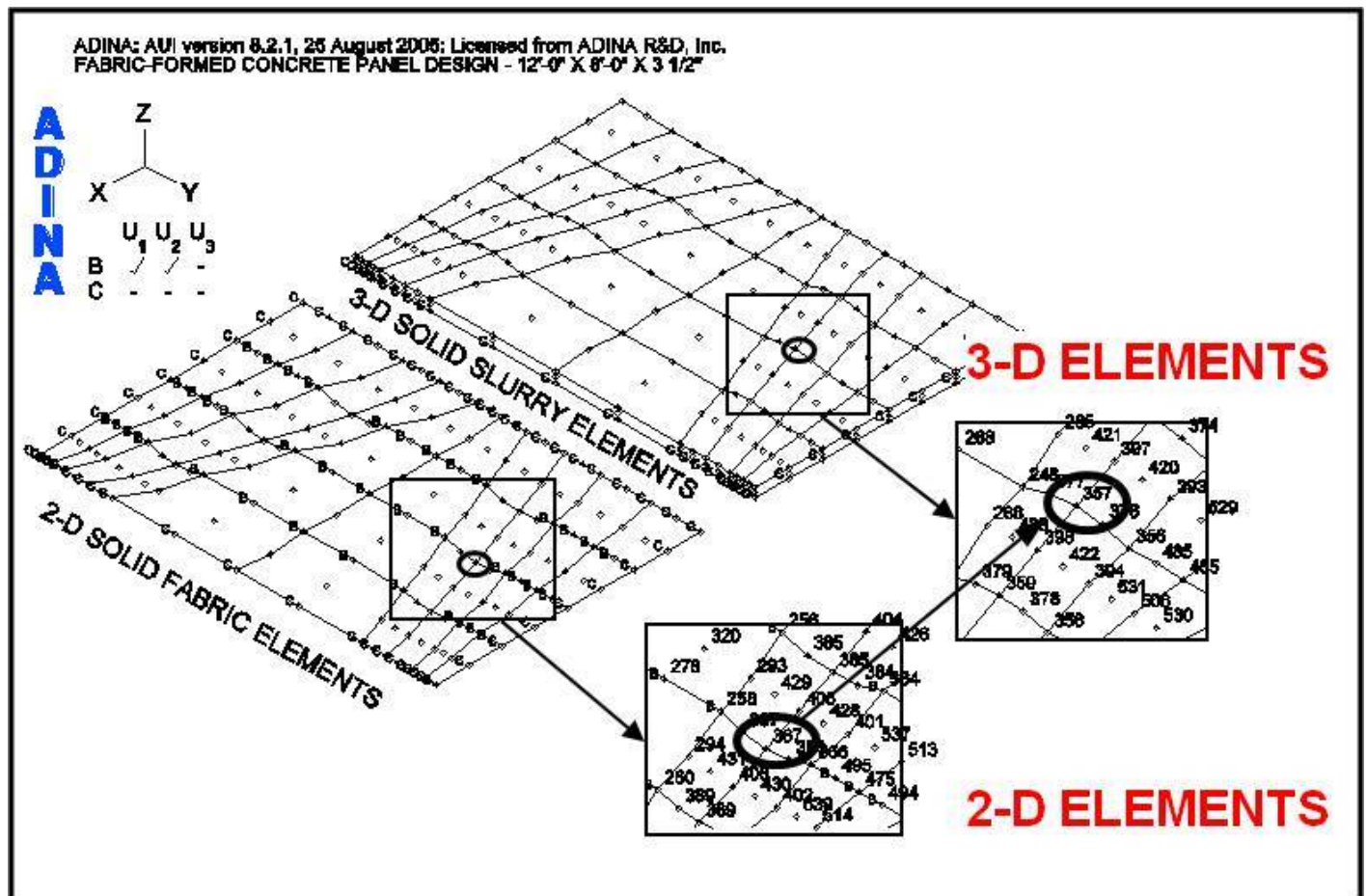
Fig. 7. "Form-finding" combined fabric and slurry model.
